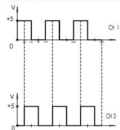
OUTPUT SIGNAL OF HALL SENSOR
